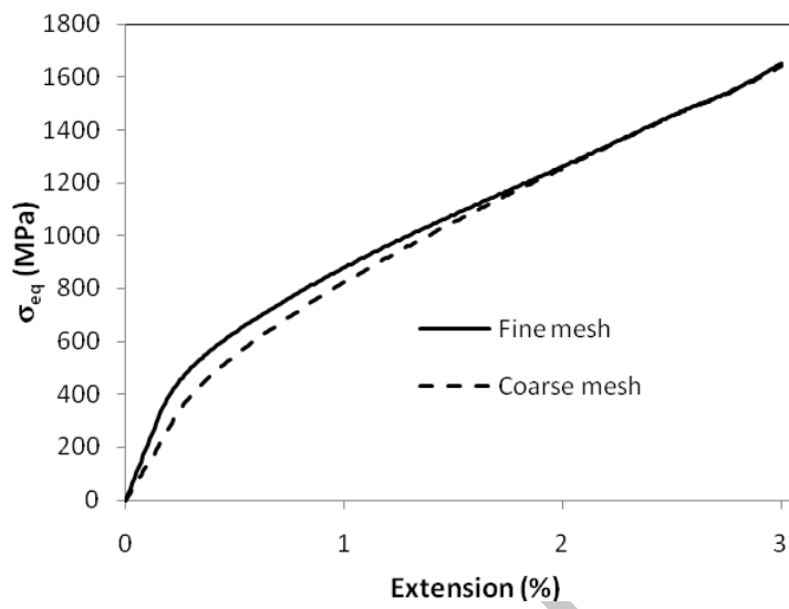
Figure 7- \sigma_q for [G_2/C_2/G_2] from fine and coarse mesh schemes
