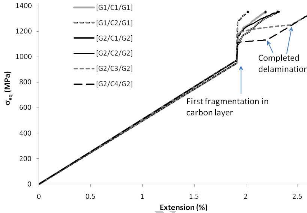
Figure 8- \sigma_q of different layups up to the predicted glass failure
