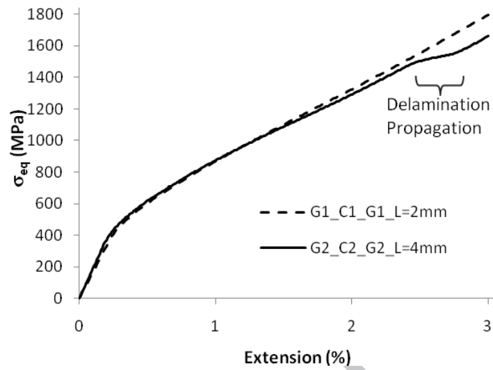
Figure 6- \sigma_q of glass layer in [G/C/G] and [G 2 /C 2 /G 2 ] laminates
