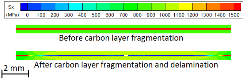
Figure 11- The stress distribution just before carbon layer fracture and after unstable delamination in the laminate [G_2/C_3/G_2]
