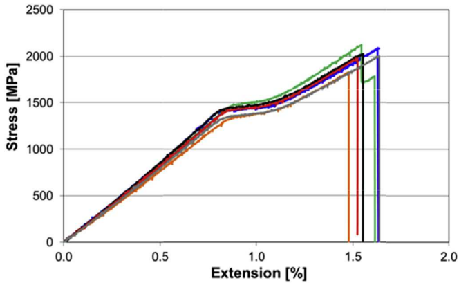
Fig. 4. Tensile response of the M55 configuration.
