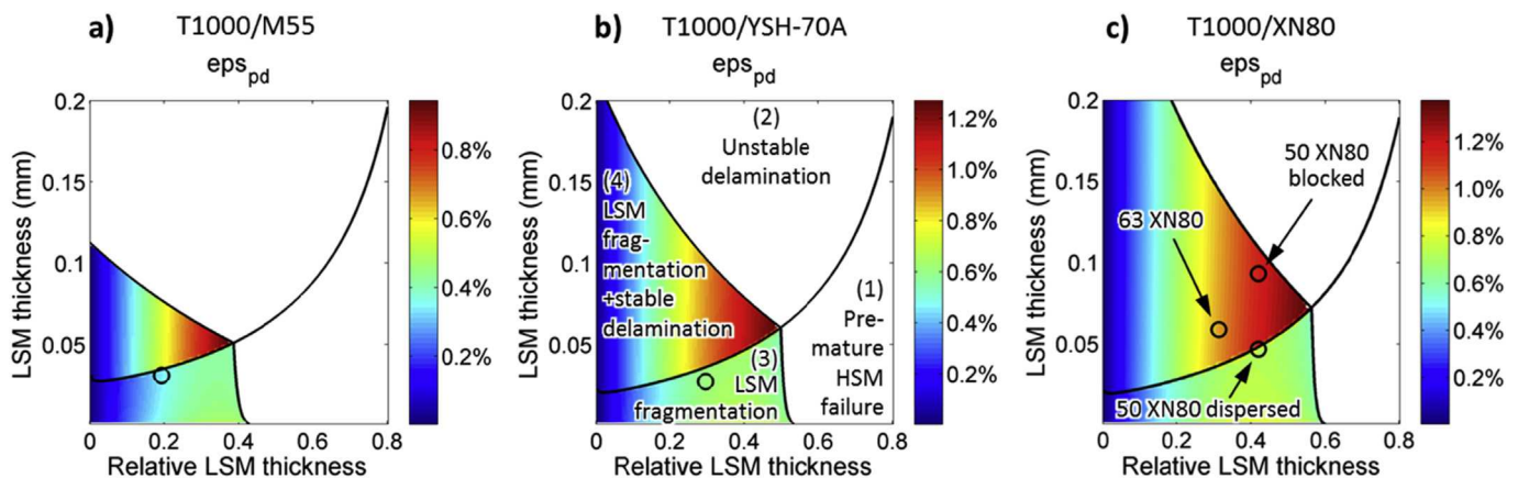
Fig. 2. Damage mode maps of the designed material combinations ( \epsilon_{psd} -pseudo-ductile strain represented by the colour palette, LSM-low strain material, HSM-high strain material, part b) indicates four regions of the map with their associated failure processes). (For interpretation of the references to colour in this figure legend, the reader is referred to the web version of this article.)
