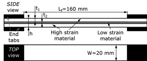
Fig. 3. Schematic of the specimen geometry.
