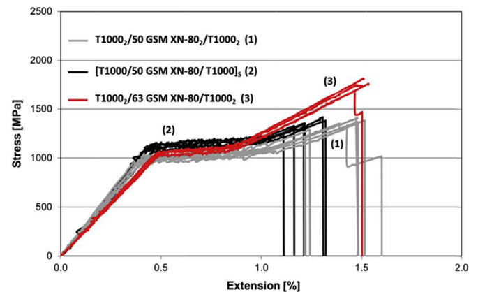
Fig. 6. Tensile response of T1000/XN-80 configurations (GSM refers to the areal density of the constituent prepreps in [g/m^2] ).
