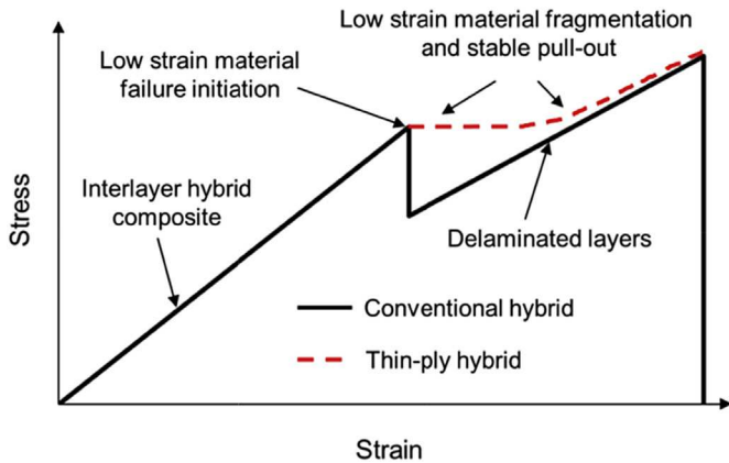
Fig. 1. Schematic of the stress-strain response of conventional and thin-ply interlayer hybrid composites.
