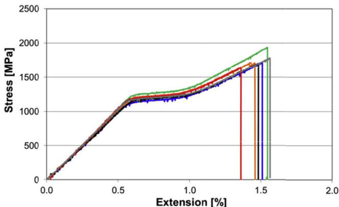
Fig. 5. Tensile response of the YSH-70A configuration.
