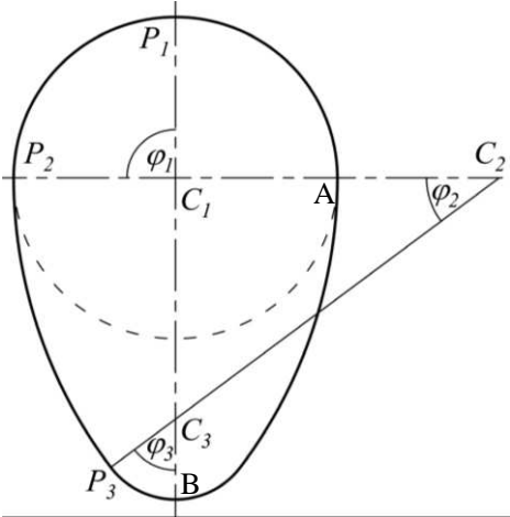
Figure 1. Cross sectional geometry of the tested and modelled egg shape profile pipes
