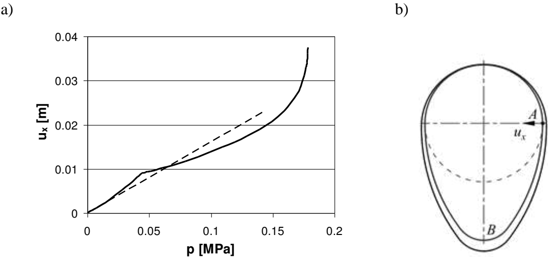
Figure 8. a) Typical outer pressure- horizontal displacement curve of a pipe-in-pipe model with a dashed line showing the initial slope b) Schematic of the displacement definition
