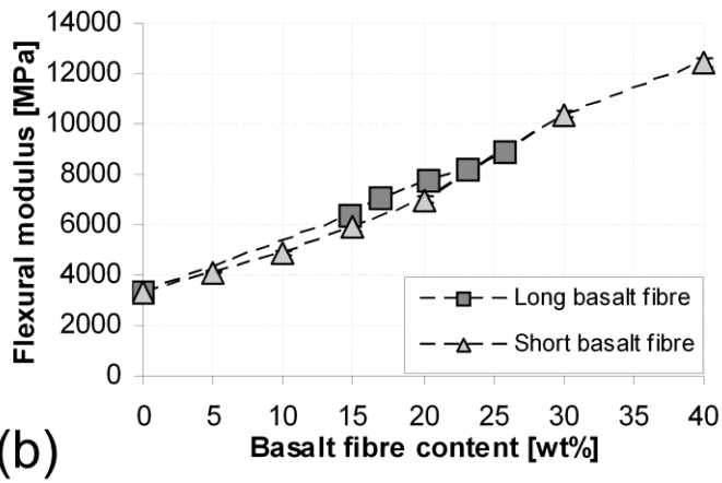
Fig. 7. Tensile (a) and flexural (b) modulus of the long and short basalt fibre reinforced PLA composites
