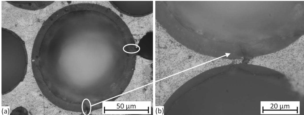
Fig. 7 SL grade hollow sphere in Al99.5 matrix (a) and magnified view of a crack (b)
