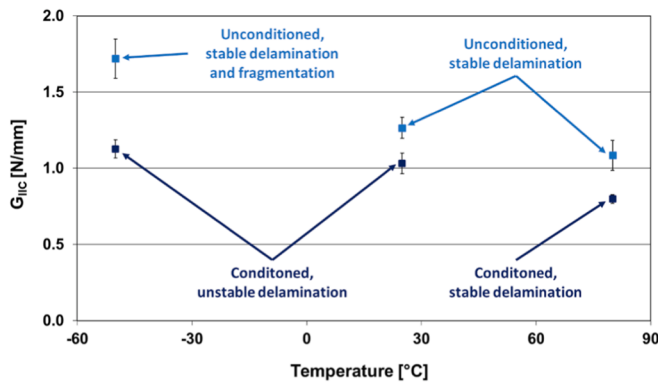
Fig. 12. The effect of test temperature and moisture on the mode II fracture toughness.
