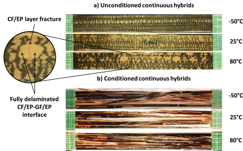
Fig. 4. Specimens with continuous carbon layer after the tensile tests: a) fragmentation of the carbon/epoxy layer and localised delamination between glass/epoxy and carbon/epoxy layers (Unconditioned), b) sudden, catastrophic failure (Conditioned).
