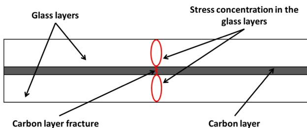
Fig. 9. Tensile stress concentration in the glass/epoxy layers in the vicinity of carbon layer fracture (delamination is neglected).
