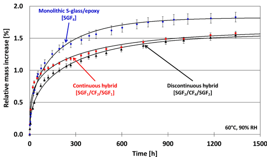
Fig. 3. Water uptake results of the continuous hybrid, discontinuous hybrid and monolithic S-glass specimens with fitted curves.
