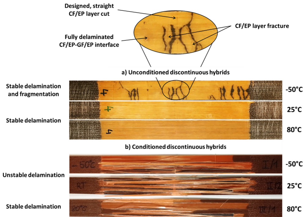
Fig. 10. Failed hybrid specimens with discontinuous CF/EP layer.
