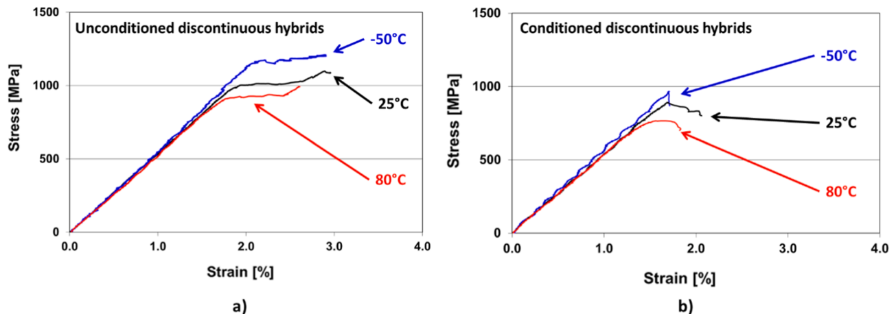
Fig. 11. Stress–strain curves of the (a) unconditioned discontinuous hybrid and (b) conditioned discontinuous hybrid specimens at various temperatures.
