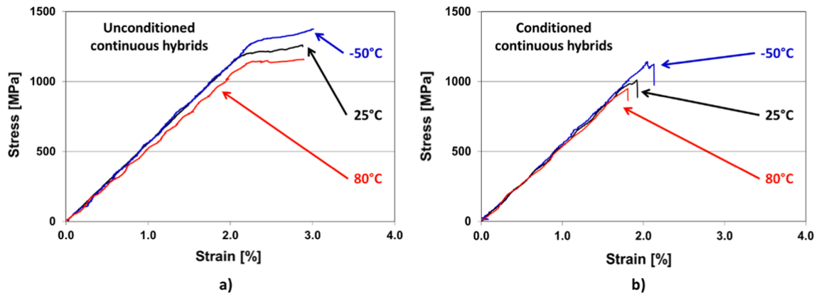
Fig. 7. Stress–strain curves of a) unconditioned continuous hybrid specimens and b) conditioned continuous hybrid specimens at all test temperatures.
