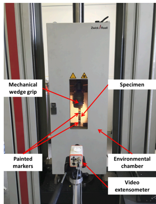
Fig. 2. Test setup.
