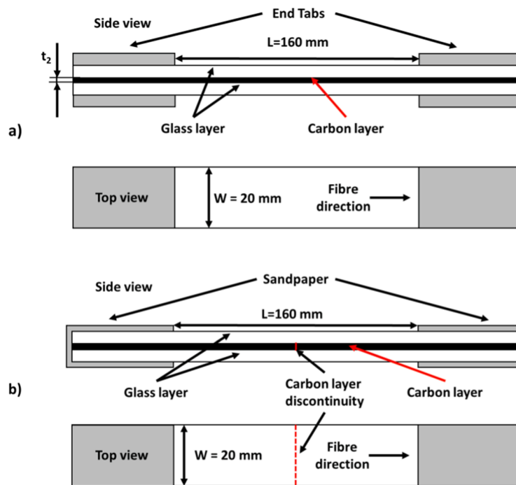
Fig. 1. Schematic of the a) continuous and b) discontinuous hybrid specimen geometry.
