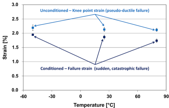
Fig. 6. Knee point strain/failure strain of continuous hybrid specimens as a function of test temperature and hot-wet conditioning.
