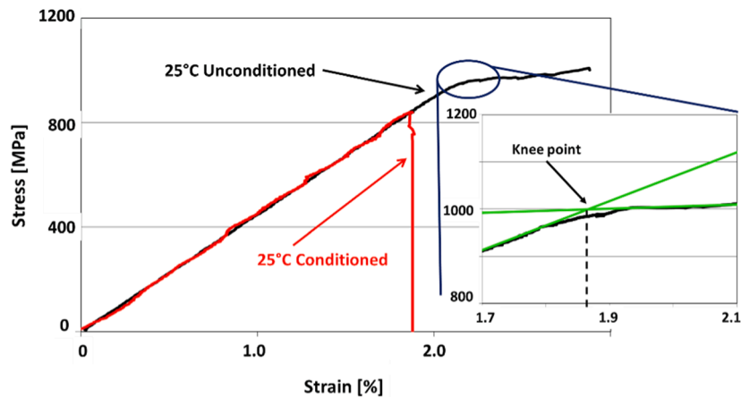
Fig. 5. The stress–strain response of typical unconditioned and conditioned continuous glass/carbon hybrid specimens and the definition of the knee point.
