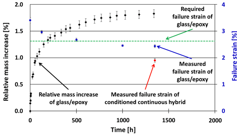
Fig. 8. Moisture induced degradation and the resulting decrease of the failure strain of UD monolithic SGF/EP specimens.
