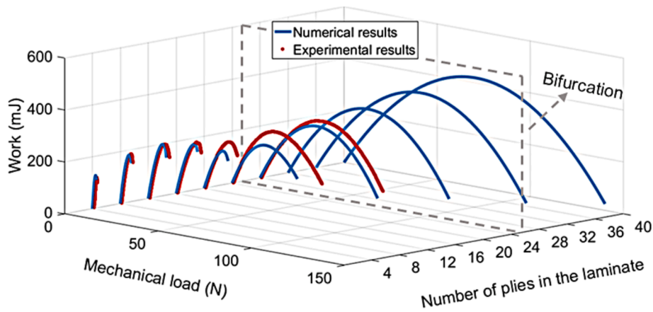
Fig. 6. Mechanical work of the loaded corner of the 190 mm × 190 mm [45 n /90 n /-75 n /-45 n ] laminates as a function of the mechanical load and the number of plies in the laminates - numerical and experimental results. Test setup: Fig. 3, bifurcation: Fig. 4.
