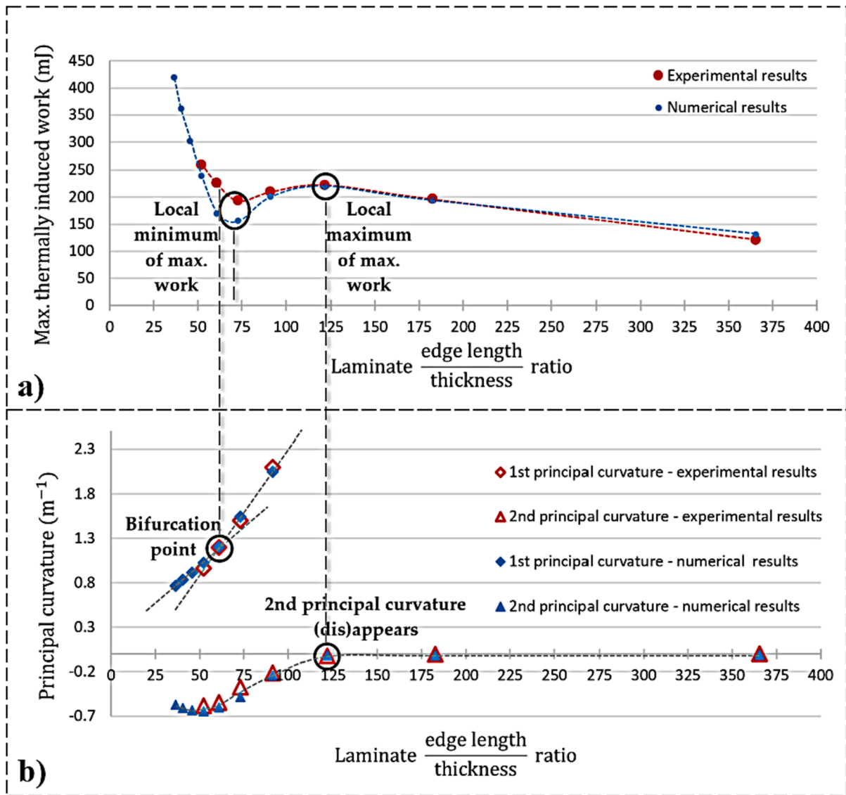
Fig. 7. Numerical and experimental results of the a) maximum thermally induced work and b) principal curvatures of the 190 mm × 190 mm [45_n/90_n/-75_n/-45_n] laminates as a function of their dimensional ratio (constant 190 mm × 190 mm laminate).
