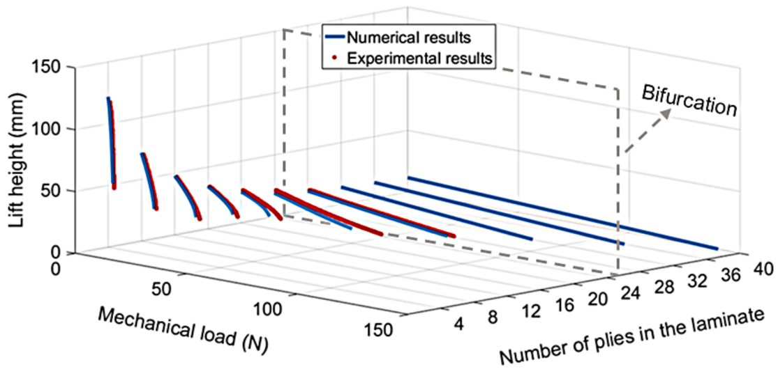
Fig. 5. Lift height of the loaded corner of the 190 mm × 190 mm [45 n /90 n /-75 n /-45 n ] laminates as a function of the mechanical load and the number of plies in the laminates - numerical and experimental results. Test setup: Fig. 3, bifurcation: Fig. 4.
