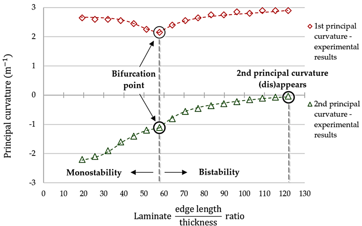
Fig. 4. Monostable-bistable transition of the [45 3 /90 3 /-75 3 /-45 3 ] laminate (constant 12-ply laminate).
