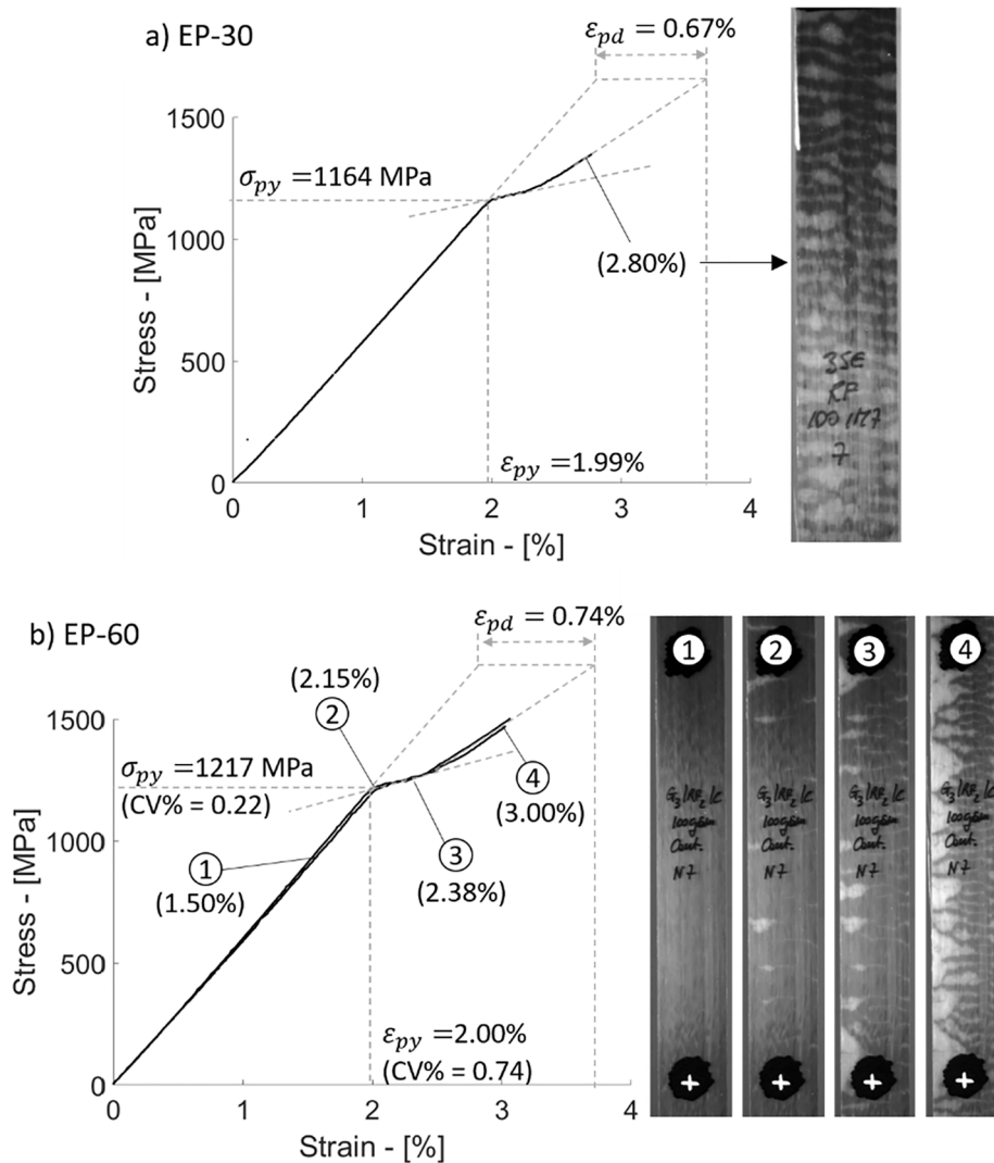
Fig. 8. Pseudo-ductile stress-strain curves of one 30 \mu\text{m} (EP-30) and one typical 60 \mu\text{m} epoxy film (EP-60) interleaved samples. The images correspond to the damage stages indicated on the stress-strain curves. (For interpretation of the references to colour in this figure legend, the reader is referred to the web version of this article.)
