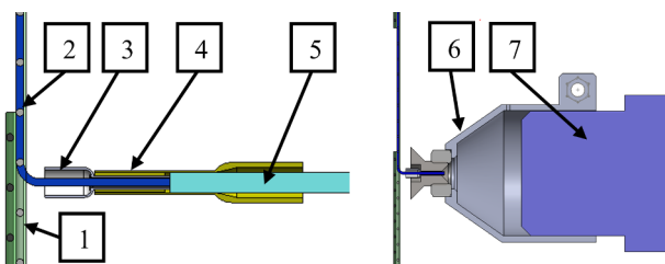
Fig. 2. Elements of connection of the fiber bundle: 1 – specimen, 2 – illuminated fiber bundle, 3 – the end of the fiber bundle in the cord-end terminal, 4 – self-made connector to connect the cord-end terminal and the optical cable, 5 – optical cable, 6 – self-made adapter to the digital microscope, 7 – lens system of the digital microscope with the connector and the specimen. (For interpretation of the references to colour in this figure legend, the reader is referred to the web version of this article.)
